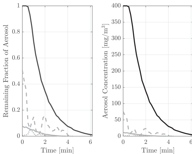
Fig. 3. Comparing different interventions at the nurses' station on aerosol clearance and transmission of aerosols. Left image shows the values normalized to the saturation value of the sensor whereas right shows the measured value. The measurements were taken with 2 air cleaners in the patient room. Note. The black solid line indicates measures taken within the patient room. The grey solid line indicates measures taken at the nurses' station (NS) with Zipwall present. The grey dashed line indicates measures taken at NS without barrier. The grey dotted line indicates measures taken at NS with air cleaner barrier present (3 air cleaners in front of desk).
